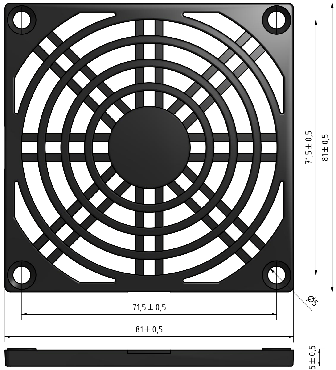
Innengitter
